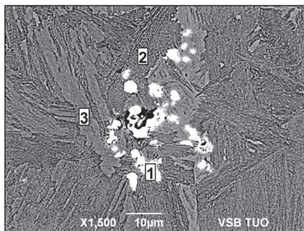
Figure 4 Microstructure of 42CrMo4 steel (with mischmetal), Scanning Electron Microscopy - SEM/EDX. 1 – inclusions, 2 – AF, 3 – M
